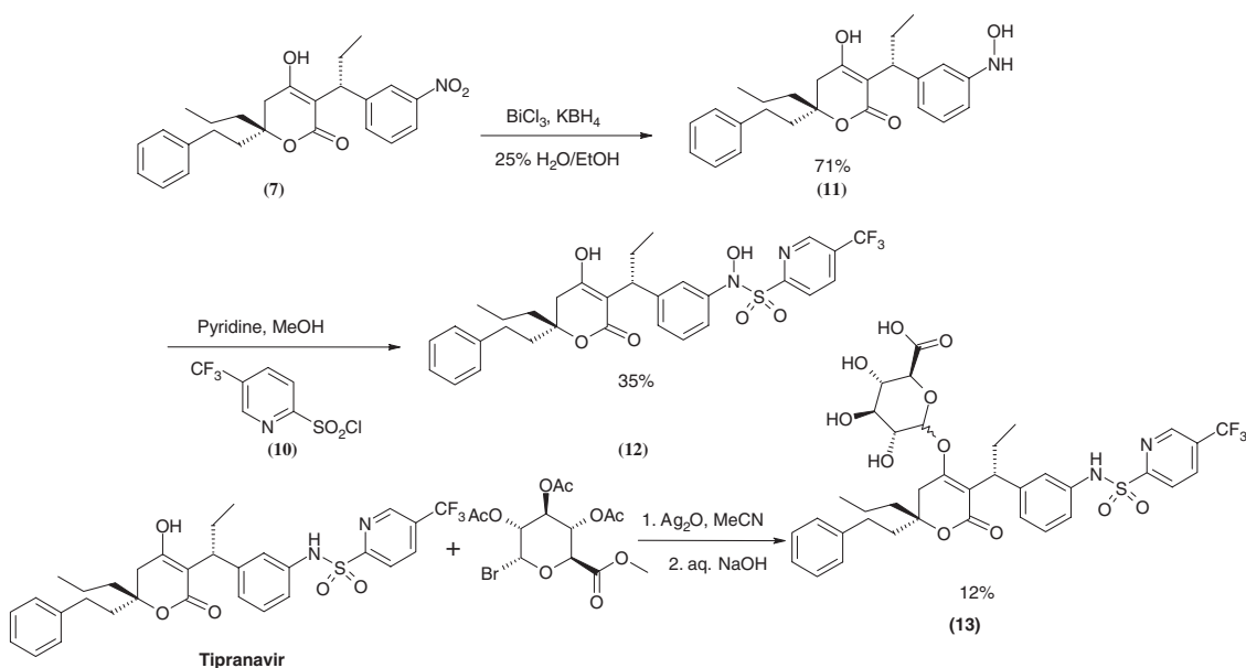
Scheme 2. Synthesis of the hydroxyl-metabolite and the glucuronide conjugate.
